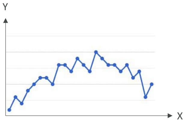
Overfitting
